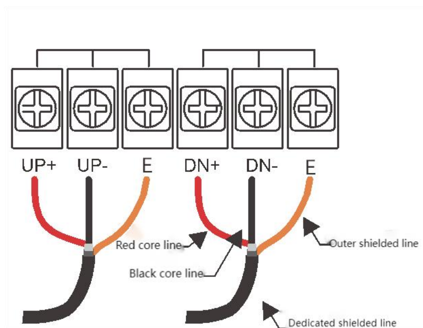
Fig.2 Sensor Connection Host
